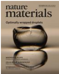
Nature Materials
