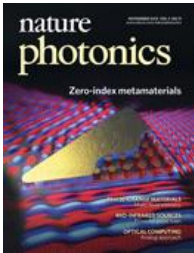
Nature Photonics
