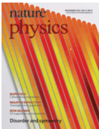
Nature Physics
